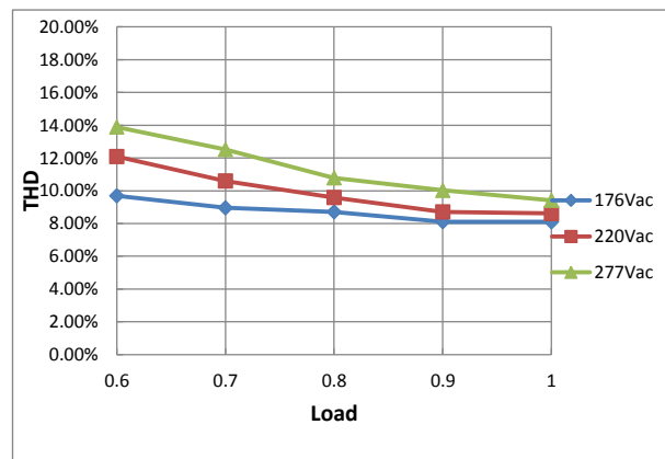
THD Curve
