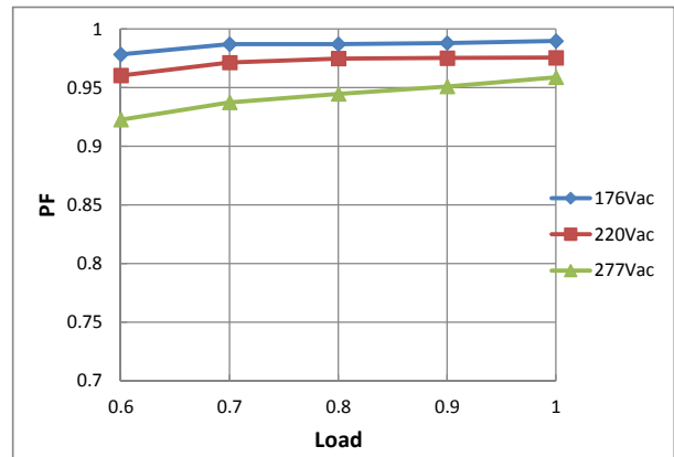
Power Factor Curve
