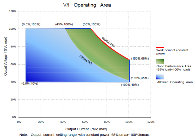
V/I Curve
